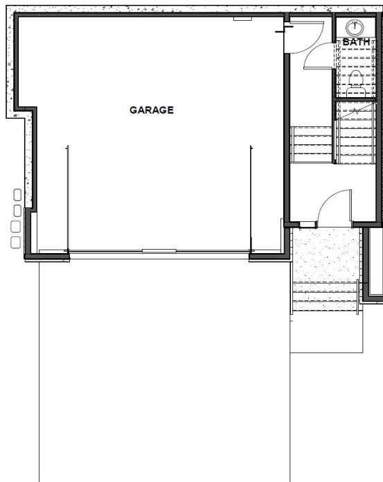
LEVEL 1
