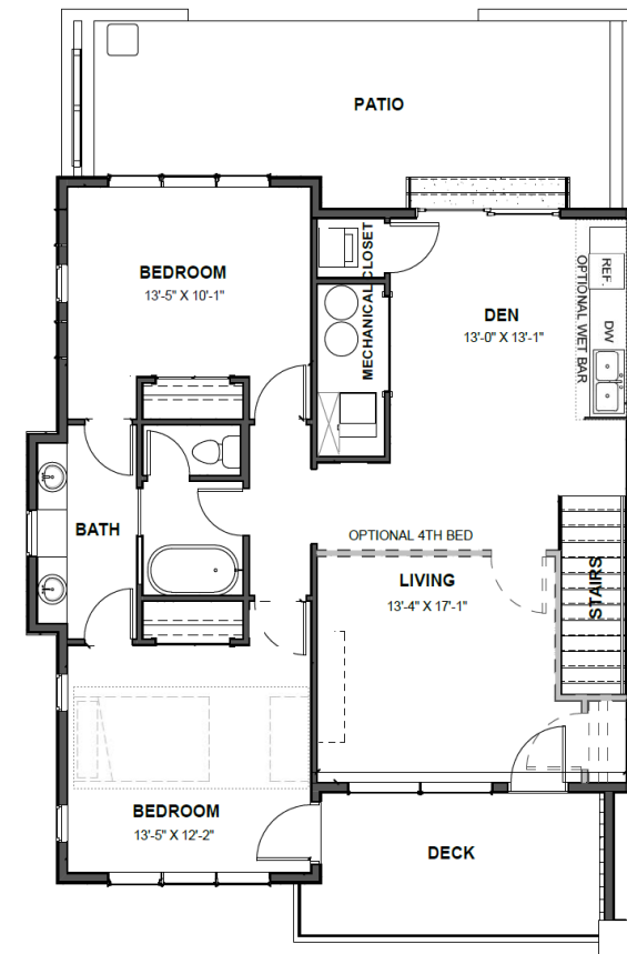
LEVEL 3
